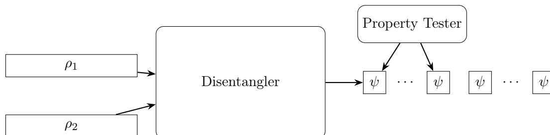
Figure 2: Schematic picture of our disentangler being used to (approximately) ensure multiple unentangled copies of a state as output. Part of these copies are used to test a given desired property. If the test passes, the remaining “certified” copies can be used in further information processing tasks.
