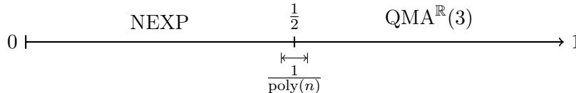
Figure 1: Gap and the complexity regime of the particular version of \text{QMA}^+(3) from Theorem 1.5 . A gap below 1/2 - 1/\text{poly}(n) corresponds to NEXP, whereas a gap above 1/2 + 1/\text{poly}(n) corresponds to \text{QMA}^{\mathbb{R}}(3) , illustrating a sharp phase transition.
